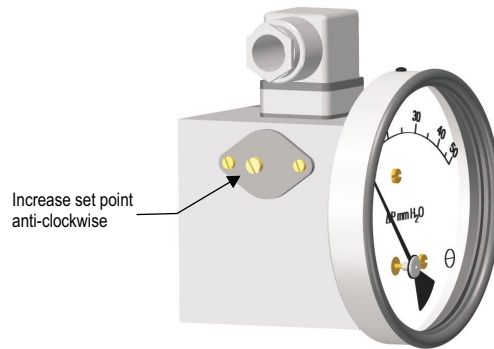
View from high pressure side
